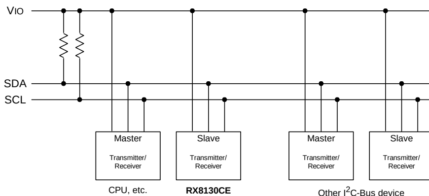
Figure 51 I 2 C-Bus connection
