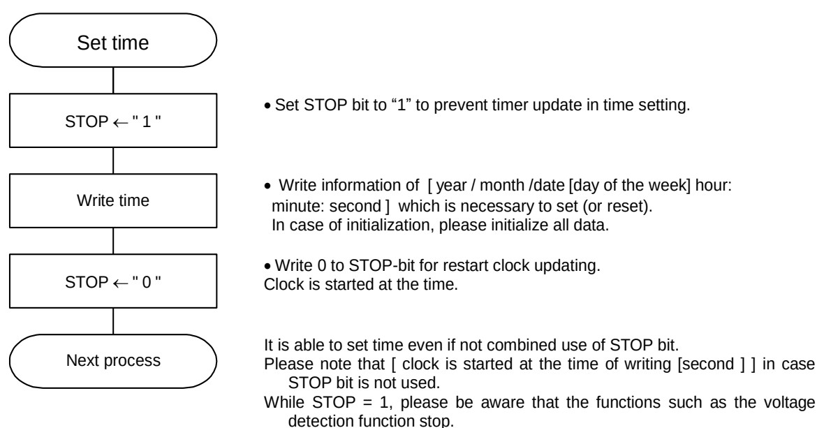
Figure 46 Example flow (Clock, calendar setting)
