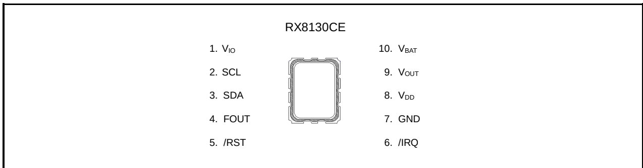
Figure 2 Package
