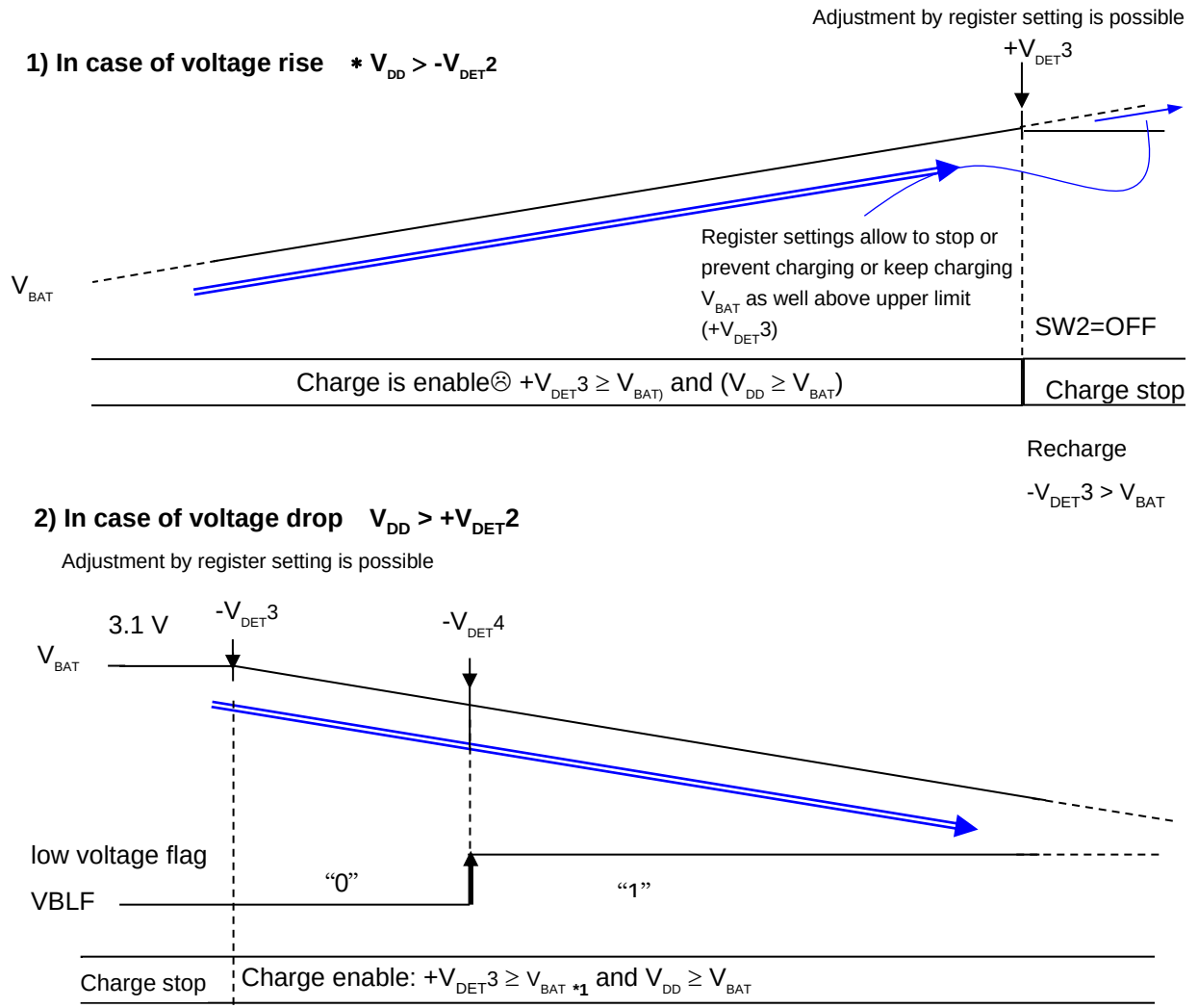
Figure 41 Re-chargeable battery operation during voltage rise and down
