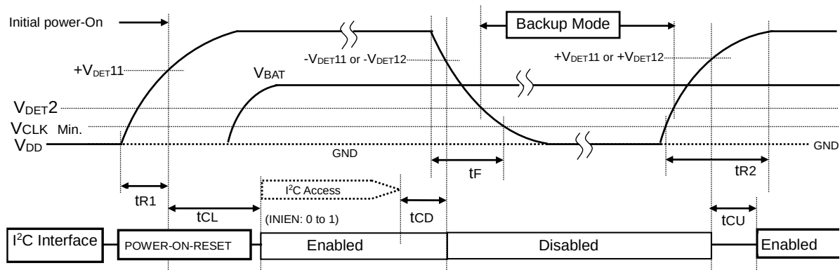
Figure 15 Power-On sequence1
