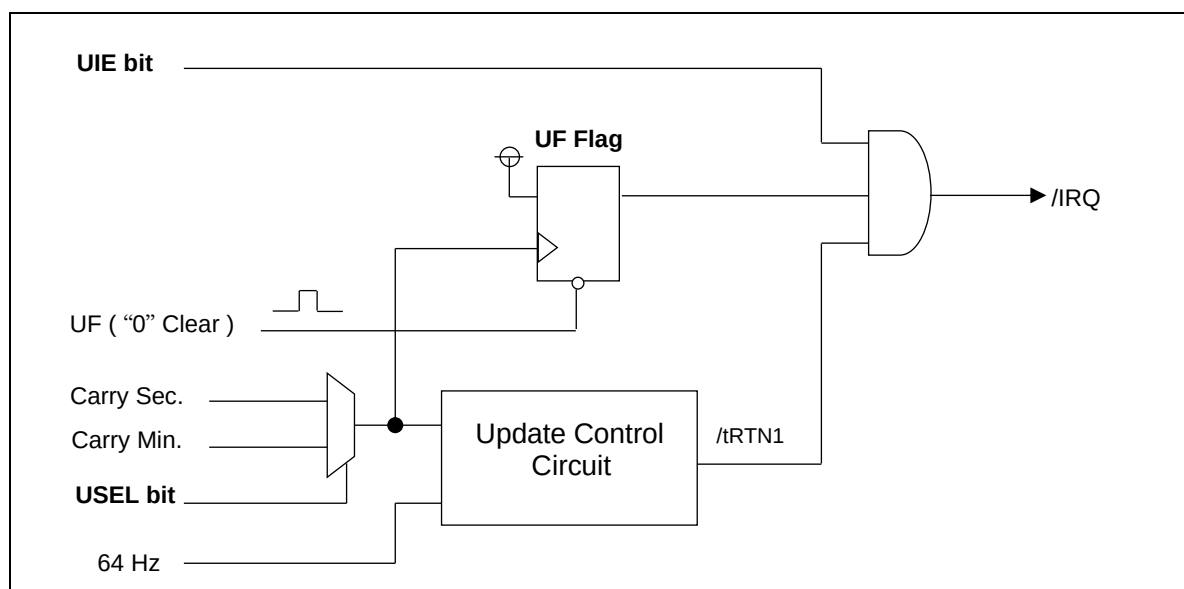
Figure 27 Time update inner block diagram
