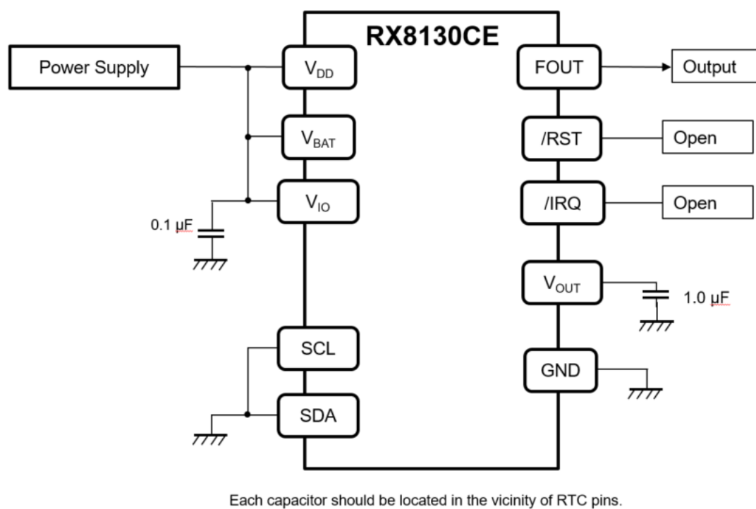
Figure 53 32.768 kHz oscillator connection
