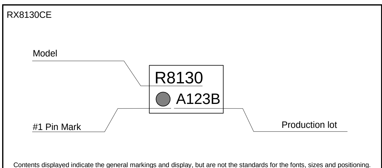
Figure 10 Marking Layout
