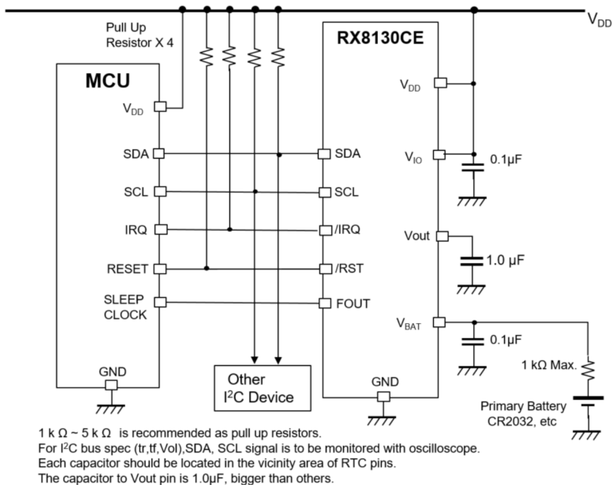
Figure 52 Typical MCU connection
