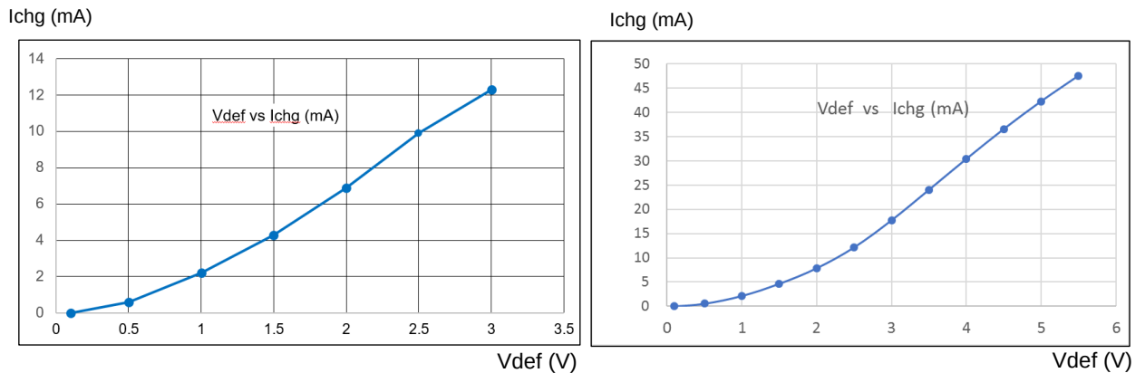
Figure 30 V_{BAT} charge current characteristics V_{DD} = 3.0\text{ V}, 5.5\text{ V}
