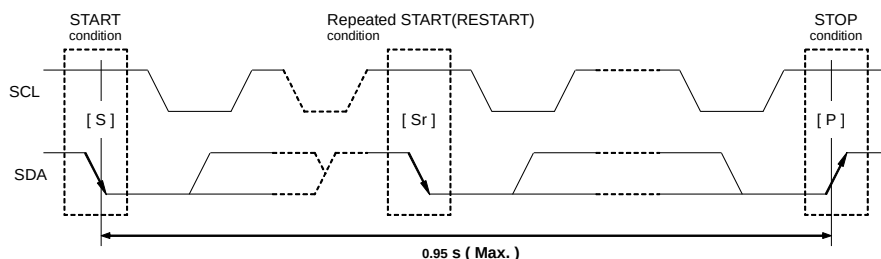
Figure 50 I 2 C-Bus start/stop timing
