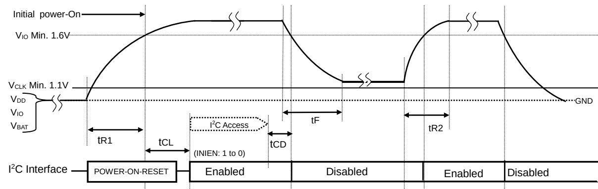
Figure 16 Power-On sequence2
