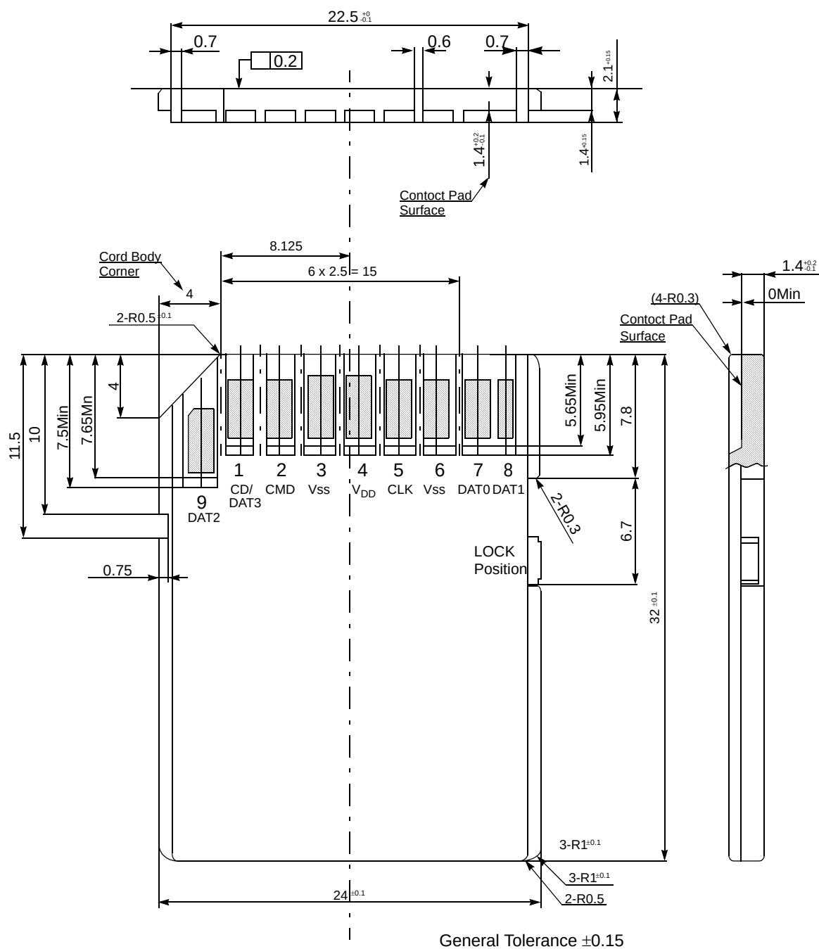
Figure 5-9. Mechanical Description
