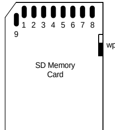
Figure 5-1. SD Memory Card shape and interface (top view)
