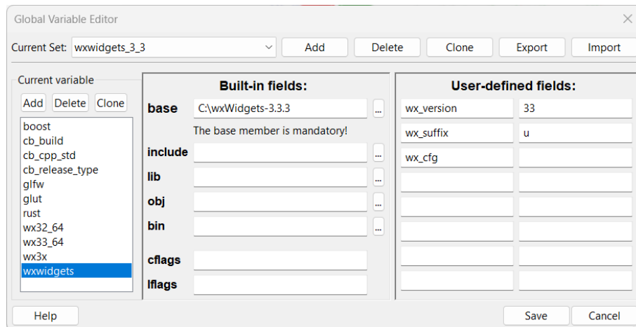
Figure 6.4: Configuring wxwidgets variable with an empty field
