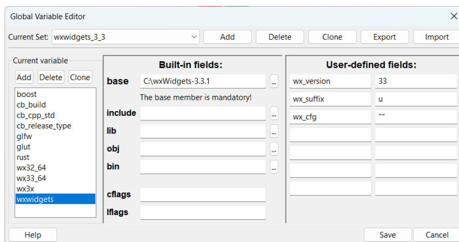
Figure 6.3: Configuring wxwidgets variable
