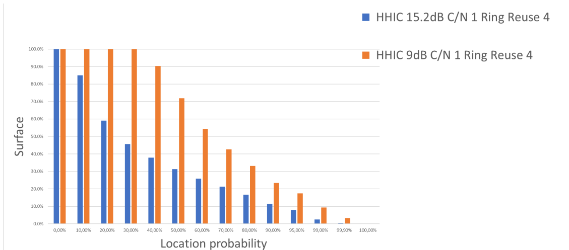
Figure 47 Handheld in car, 15.2 dB/9dB SINR, 1 additional ring
