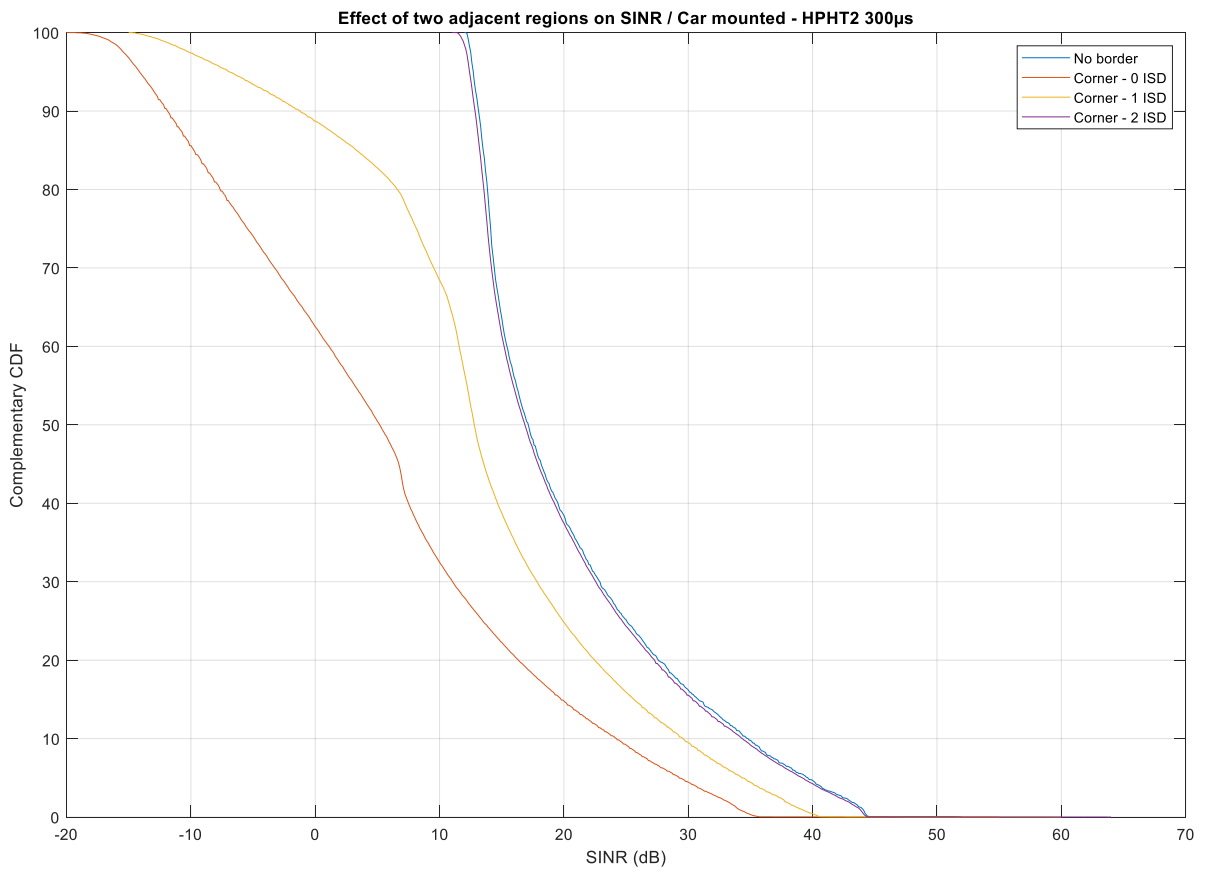
Figure B1 Corner regional boundary results for HPHT
