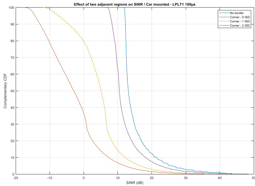
Figure 15 CDF for LPLT corner regional boundary
