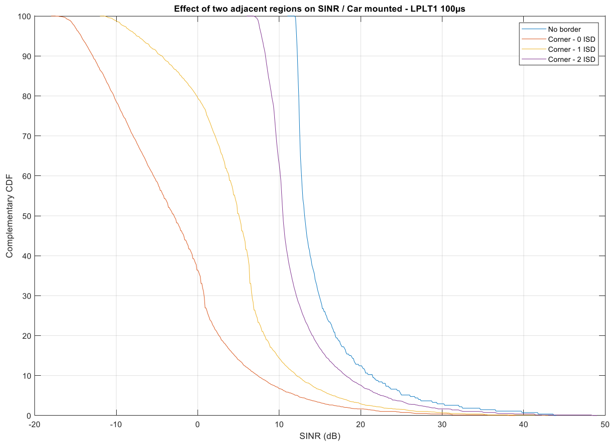
Figure B7 Corner regional boundary results for LPLT
