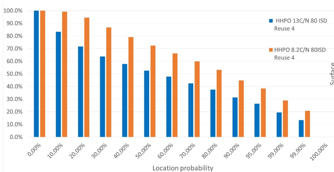
Figure 43 Handheld portable outdoor, 8.2dB/13dB SINR, 80 km ISD
