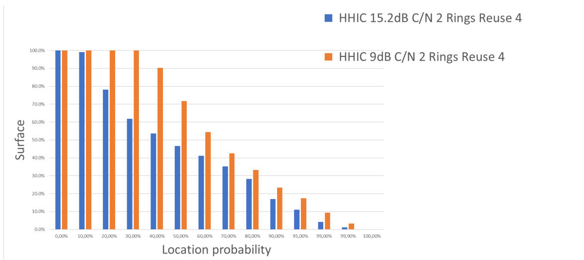
Figure 50 Handheld in car, 15.2dB/9dB SINR, 2 additional rings
