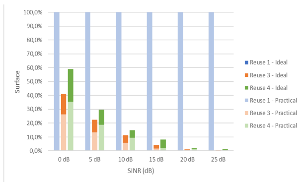
Car Mounted - LPLT Suburban - 100µs CP Ideal vs Practical
