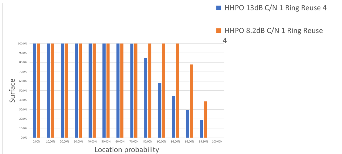
Figure 46 Handheld portable outdoor, 13dB/8.2dB SINR, 1 additional ring
