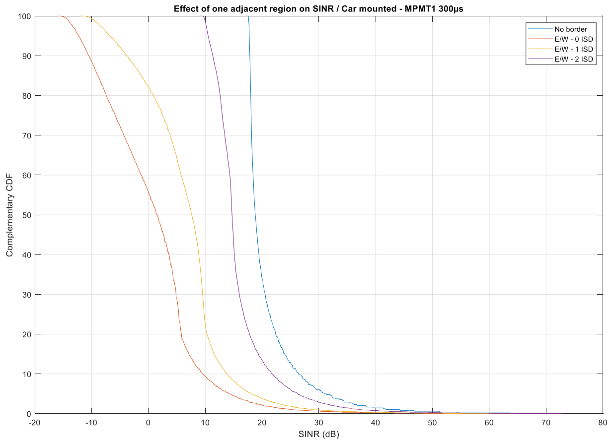
Figure B5 Straight E/W boundary region results comparison for MPMT
