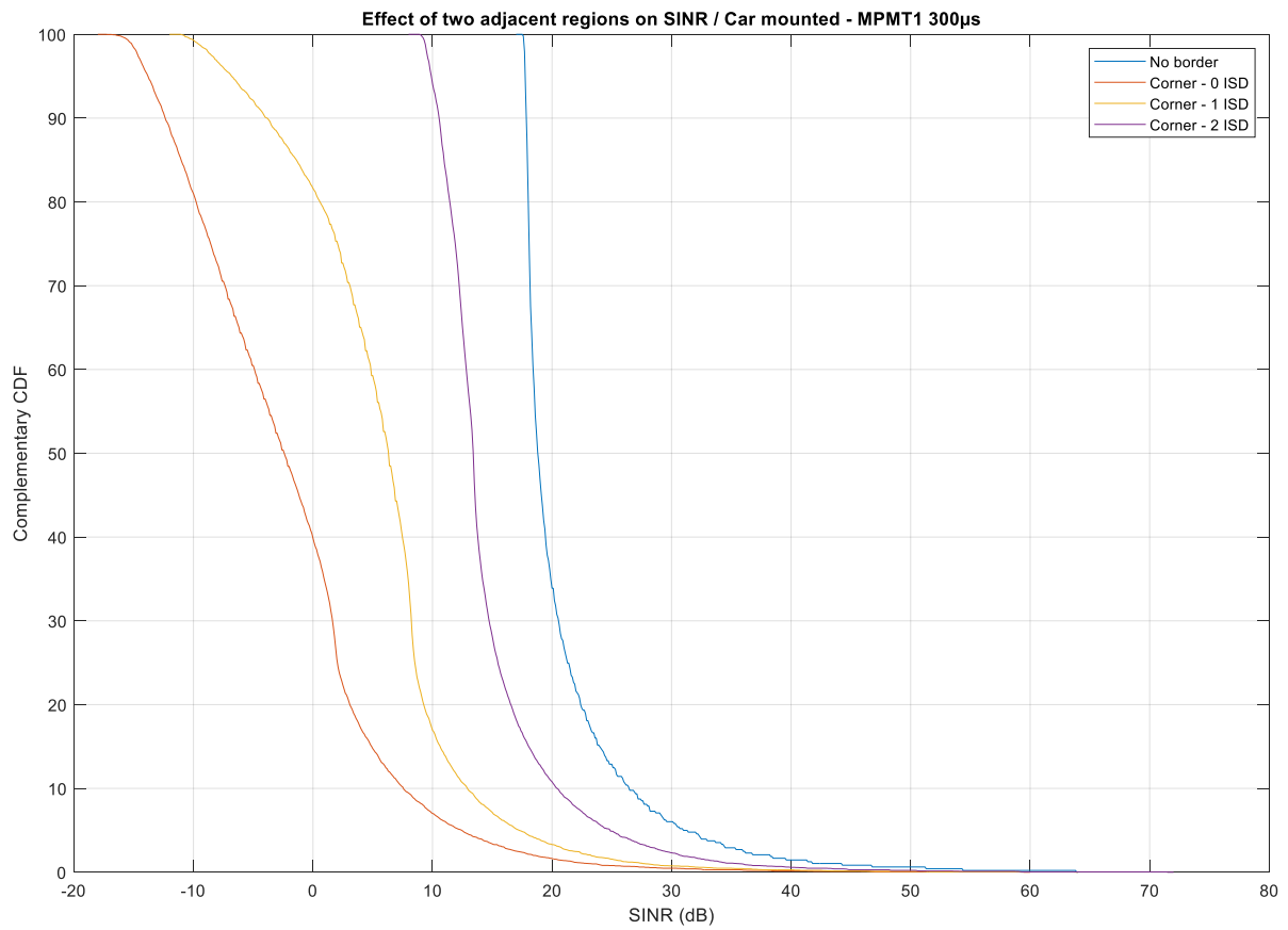
Figure B4 Regional boundary results for MPMT
