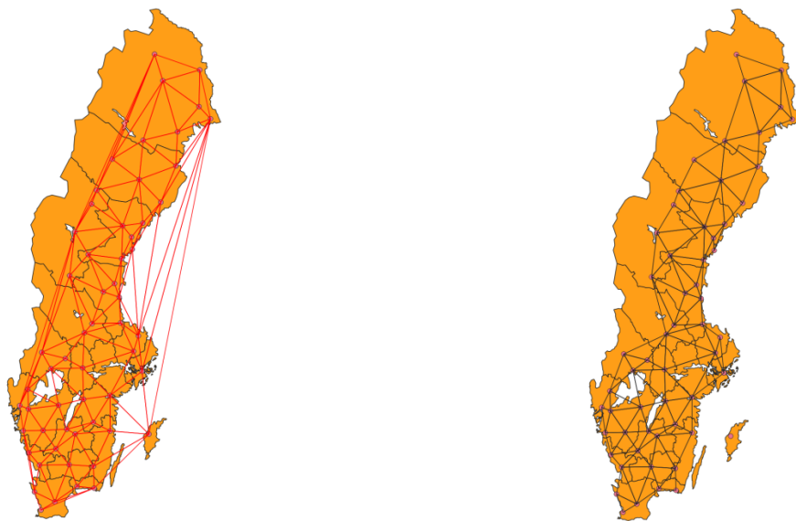
Full Delaunay Triangulation
