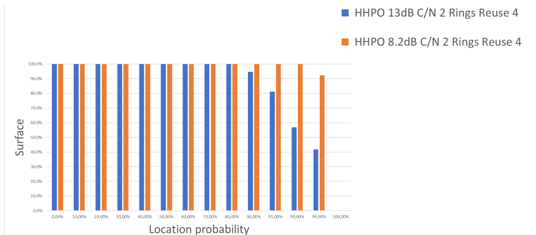
Figure 49 Handheld portable outdoor, 13dB/8.2 dB SINR, 2 additional rings
