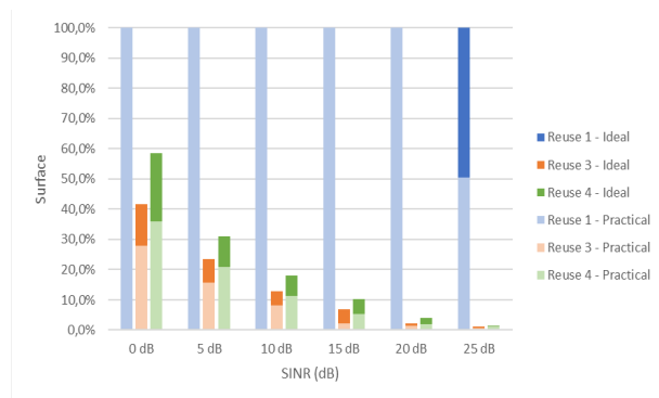
Car Mounted - LPLT Urban - 100µs CP Ideal vs Practical
