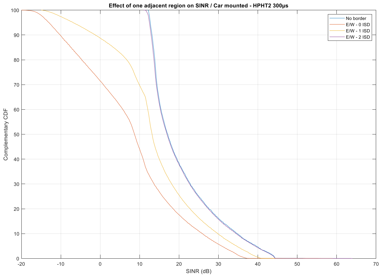
Figure B2 Straight E/W boundary region results comparison for HPHT
