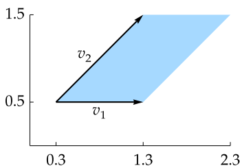
The parallelepiped (0.3, 0.5) + P((1, 0), (1, 1)) in \mathbf{R}^2 .
