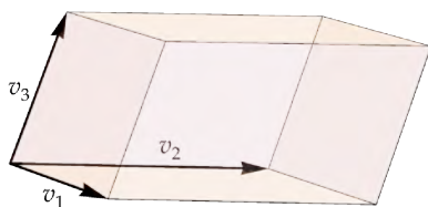
A parallelepiped in \mathbf{R}^3 .
