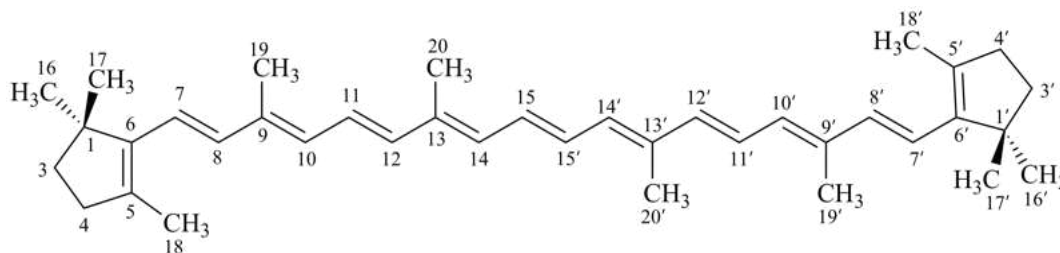
2,2'-dinor-β,β-carotene
