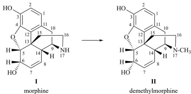
I (5 β H)-17-methyl-7,8-didehydrofuro[2',3',4',5':4,12,13,5]morphinan-3,6 α -diol II (5 β H)-7,8-didehydrofuro[2',3',4',5':4,12,13,5]morphinan-3,6 α -diol
