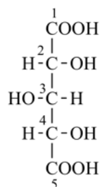
meso -xylaric acid
