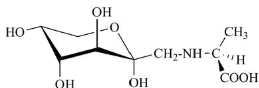
N -(1-deoxy- \alpha -D-fructopyranos-1-yl)-L-alanine
