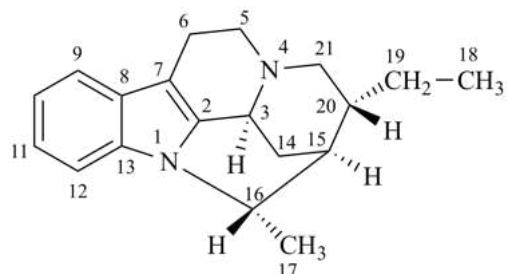
(16 \beta H )-1,16-cyclocorynan
