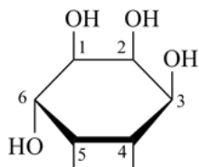
neo -inositol (1,2,3/4,5,6-)
