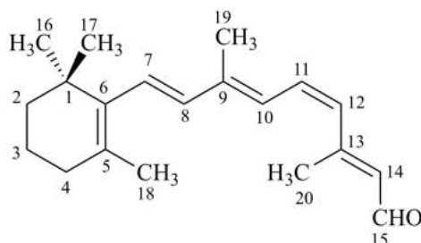
11- cis -retinal
