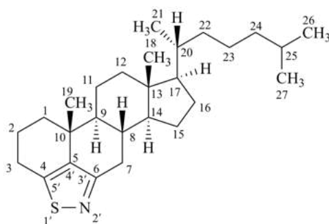
[1,2]thiazolo[5',4',3':4,5,6]cholestane (not isothiazolo[5',4',3':4,5,6]cholestane;
