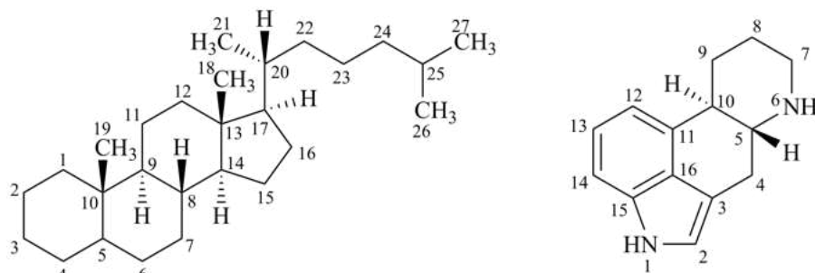
cholestane
