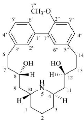
6'-deoxylythranidine
