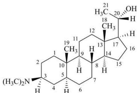
(20 S )-3 \beta -(dimethylamino)-5 \alpha -pregnan-20-ol
