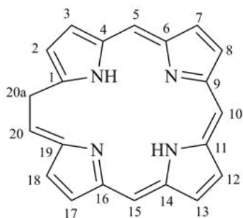
(A) 20aH-20a-homoporphyrin
