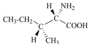
L-alloisoleucine (symbol 'alle') (2 S ,3 R )-2-amino-3-methylpentanoic acid
