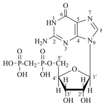
guanosine 5'-[hydrogen (phosphonomethyl)phosphonate] guanosine 5'-(tri-hydrogen methylenediphosphate) guanosine 5'-(tri-hydrogen 2-carbadiphosphate) (this name preserves the integrity of the nucleotide name; see P-101.4.3)
