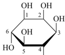
myo -inositol (1,2,3,5/4,6-)
