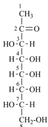
1-deoxy-L-glycero-D-alto-oct-2-ulose (3 S ,4 R ,5 R ,6 R ,7 S )-3,4,5,6,7,8-hexahydroxyoctan-2-one
