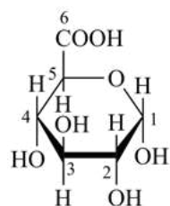
\alpha -D-glucopyranuronic acid
