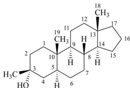
3 \beta -methyl-5 \alpha -androstan-3 \alpha -ol
