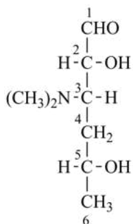
3,4,6-trideoxy-3-(dimethylamino)-D-xylulose (2 R ,3 S ,5 R )-3-(dimethylamino)-2,5-dihydroxyhexanal
