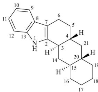
(4 \beta H)-4-carbayohimban
