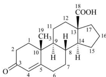
3-oxoandrost-4-en-18-oic acid
