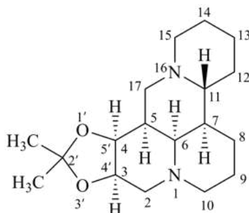
(3α H ,4α H )-2',2'-dimethyl-3,4-dihydro[1,3]dioxolo[4',5':3,4]matridine propan-2-one matridine-3β,4β-diyl ketal (see P-66.6.5) acetone matridine-3β,4β-diyl ketal
