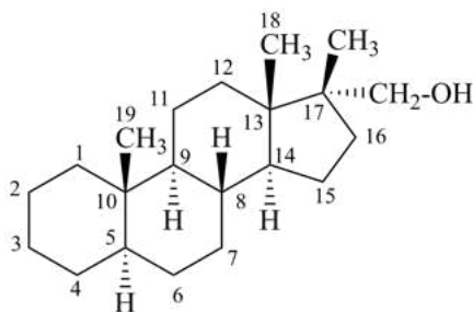
(17 \beta -methyl-5 \alpha -androstan-17 \alpha -yl)methanol
