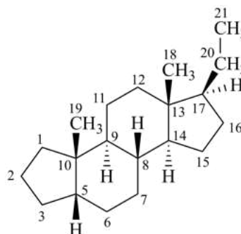
4-nor-5β-pregnane
