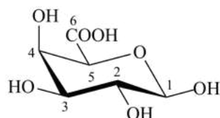
\beta -D-galactopyranuronic acid
