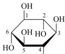
scyllo -inositol (1,3,5/2,4,6-)
