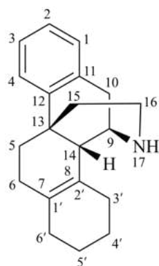
3',4',5',6'-tetrahydrobenzo[7,8]morphinan
