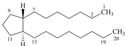
prostane (fundamental parent structure)
