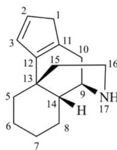
1 H -4-normorphinan
