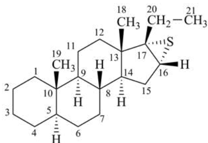
3 \alpha ,8-epidioxy-5 \alpha ,8 \alpha -androstane
