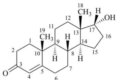
17 \alpha -hydroxyandrost-4-en-3-one
