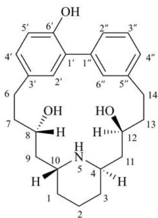
2''-demethoxylythranidine
