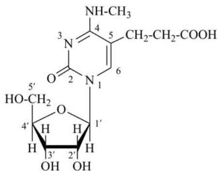
3-[4-(methylamino)-2-oxo-1-β-D-ribofuranosyl-1,2-dihydropyrimidin-5-yl]propanoic acid
