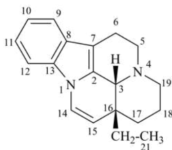
eburnamenine (fundamental parent structure)
