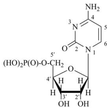
5'-cytidylic acid
