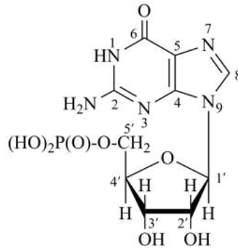
5'-guanylic acid
