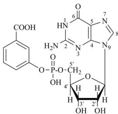
3-(5'-guanylyloxy)benzoic acid
