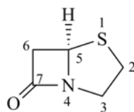
penam (fundamental parent structure) (note new numbering)
