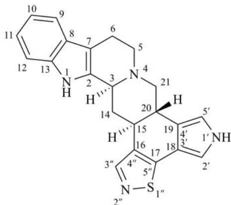
1'H-pyrrolo[3',4':18,19][1,2]thiazolo[4'',5'':16,17]yohimban
