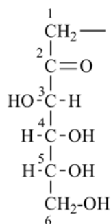
1-deoxy-D-fructos-1-yl
