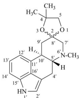
(2 \xi )-4,4,6'-trimethylspiro[1,3-dioxolane-2,8'-ergoline]
