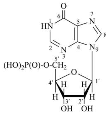
5'-inosinic acid
