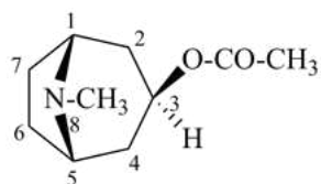
tropan-3β-yl acetate (1 R ,3 s ,5 S )-8-methyl-8-azabicyclo[3.2.1]octan-3-yl acetate (see P-93.5.2.2.1)
