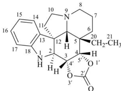
(3β H ,4β H )-3,4-dihydro[1,3]dioxolo[4',5':3,4]aspidospermidin-2'-one aspidospermidine-3α,4α-diyl carbonate (see P-65.6.3.5.4)
