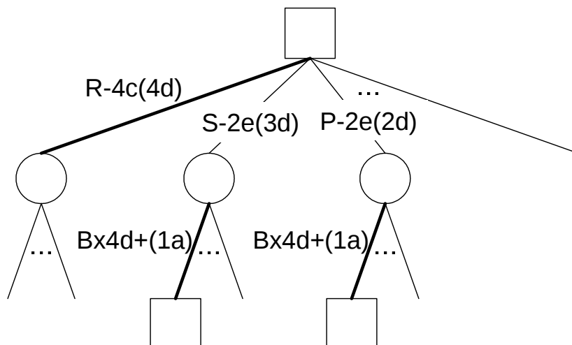
Figure 2.14: An illustration of killer move heuristics
