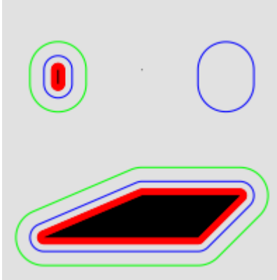
Fig. 23: Geomtransform buffer
