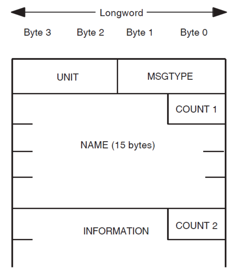
Figure D.1. Mailbox Message Structure
