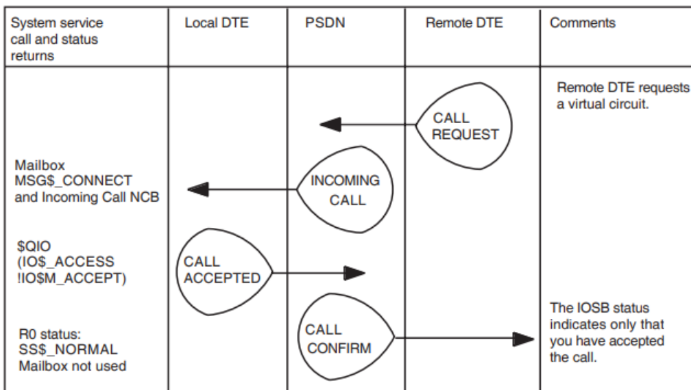
Figure 3.5. Accept a Request to Set Up a Virtual
