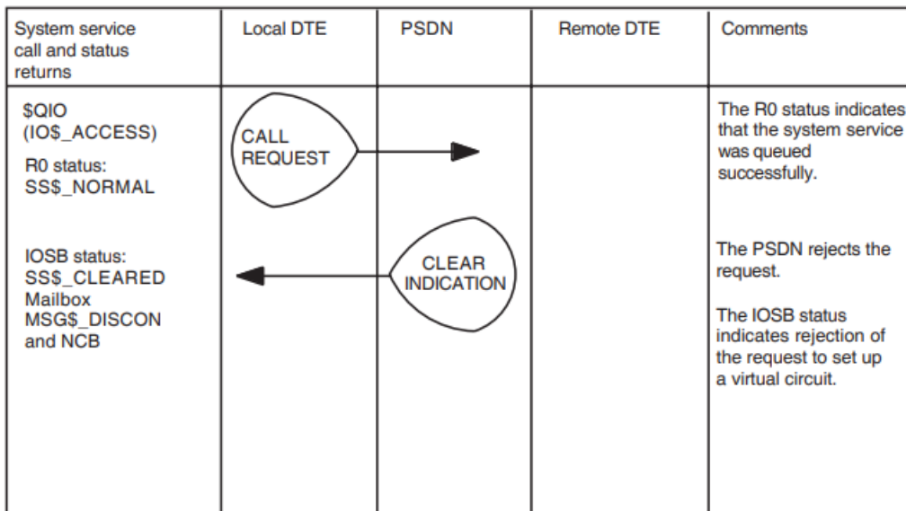
Figure 3.3. Set Up a Virtual Circuit -Call Rejected by Network
