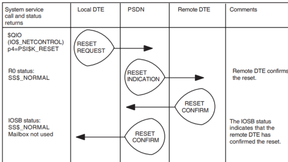
Figure 3.11. Reset a Virtual Circuit
