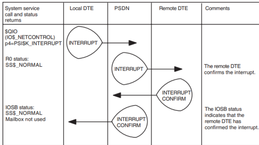
Figure 3.10. Confirm Receipt of an Interrupt
