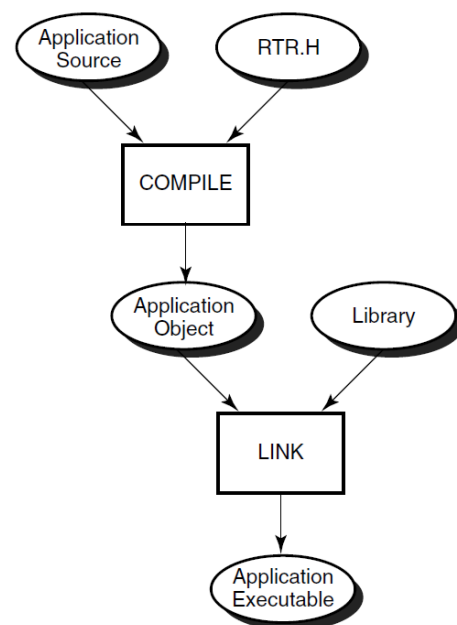
Figure 4.1. Compile Sequence
