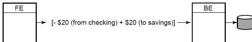
Figure 3.5. Transactional Messaging
