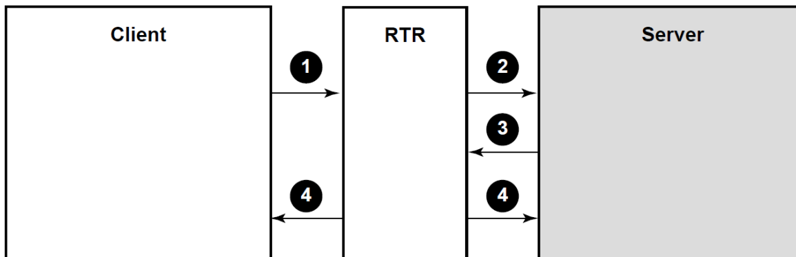
Figure 4.4. Accept Processing
