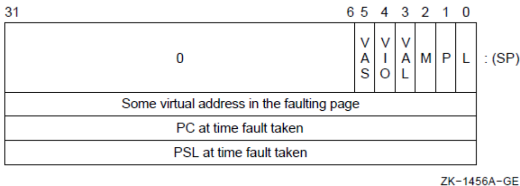
Figure 10.12. Memory Management Fault Stack Frame (as Sent by the Vector Processor)
