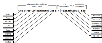
Figure 9.1. Time Display Format
