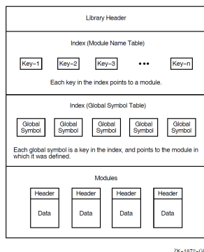
Figure 13.2. Structure of an Object or Shareable Image Library
