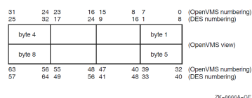
Figure 11.2. NBS Numbering Overlay on an OpenVMS Quadword
