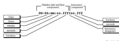
Figure 9.3. Relative Time Syntax
