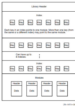
Figure 13.3. Structure of a User-Developed Library
