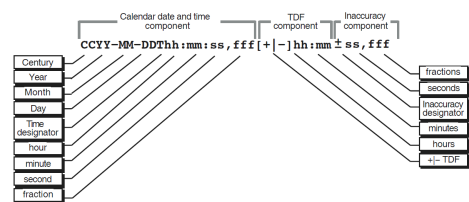
Figure 9.2. Time Display Format Variants
