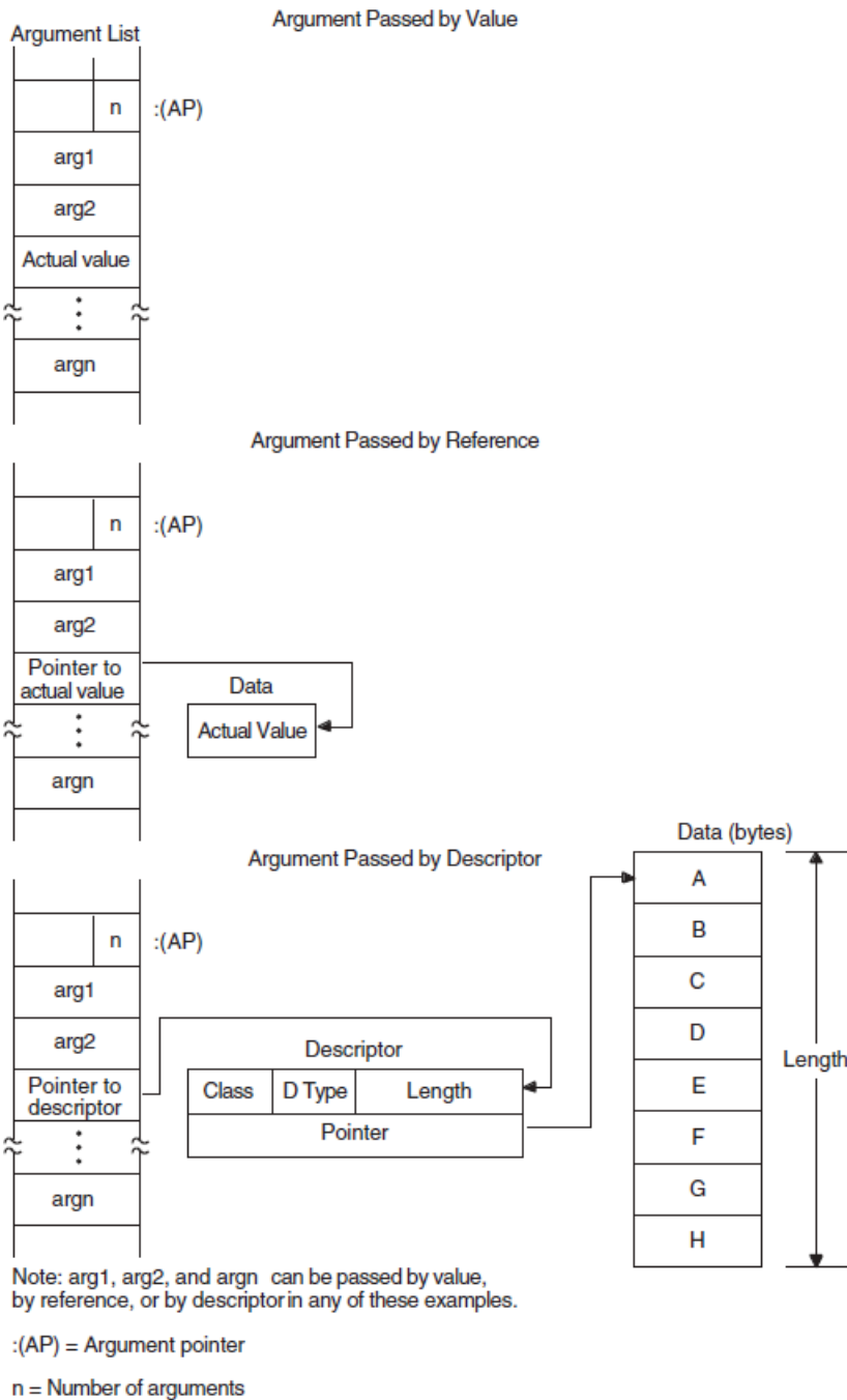
Figure 2.15. VAX Procedure Argument-Passing Mechanisms
