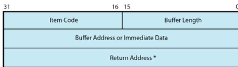
Figure 5.4. Itemlist Read Descriptor
