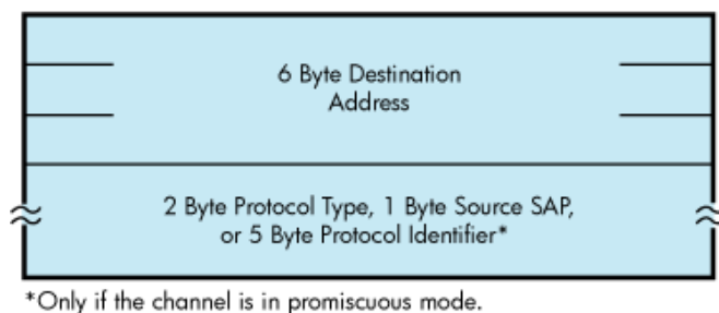
Figure 9.13. Write Function P5 Buffer
