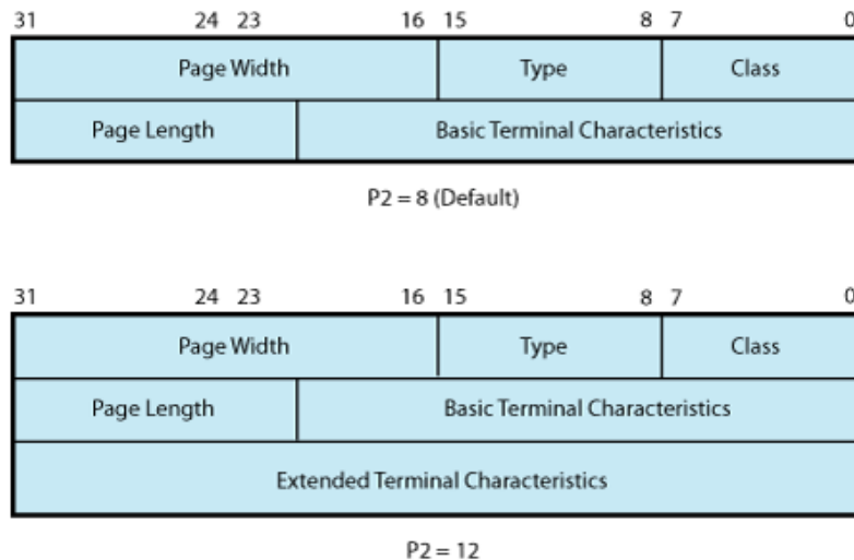
Figure 5.7. Set Mode and Set Characteristics Buffers
