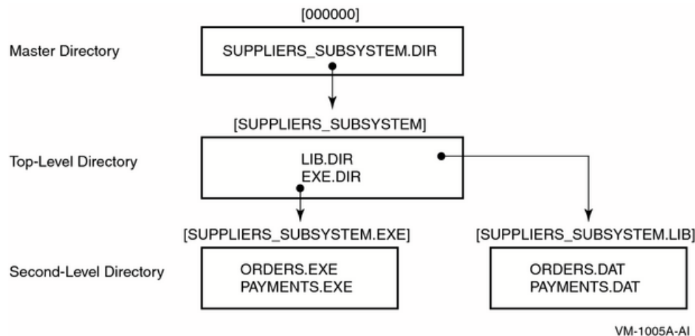
Figure 14.2. Directory Structure of the Taylor Company's Subsystem
