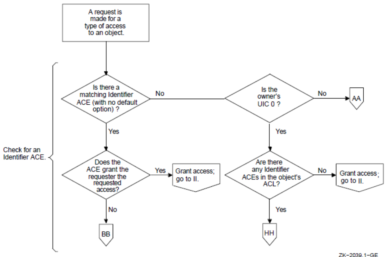
Figure 4.3. Flowchart of Access Request Evaluation
