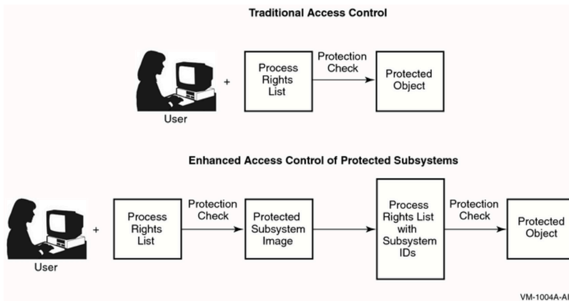
Figure 14.1. How Protected Subsystems Differ from Normal Access Control
