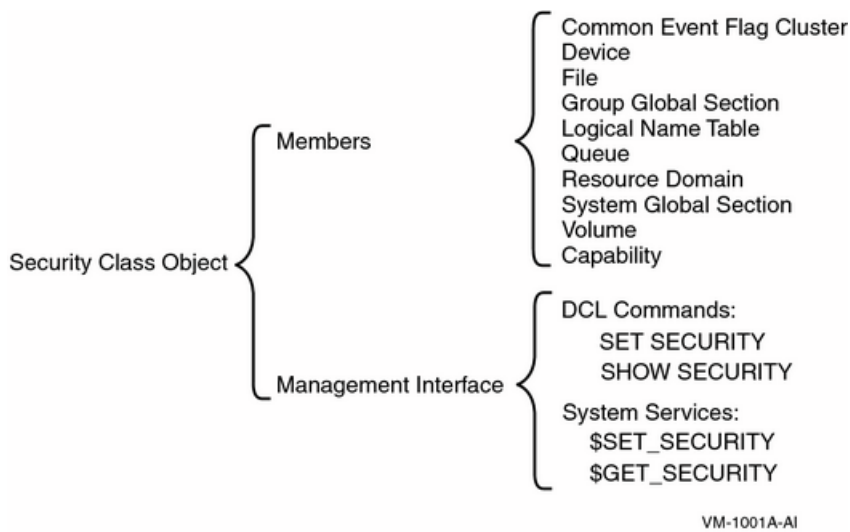
Figure 8.2. Security Class Object
