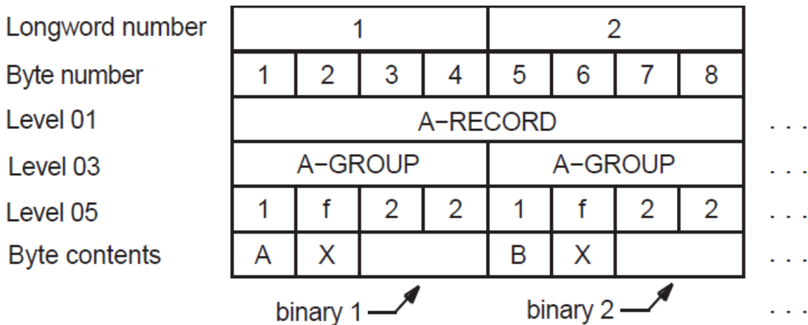
Figure 4.11. Memory Map for Example 4.13, "Initializing Mixed Usage Items"
