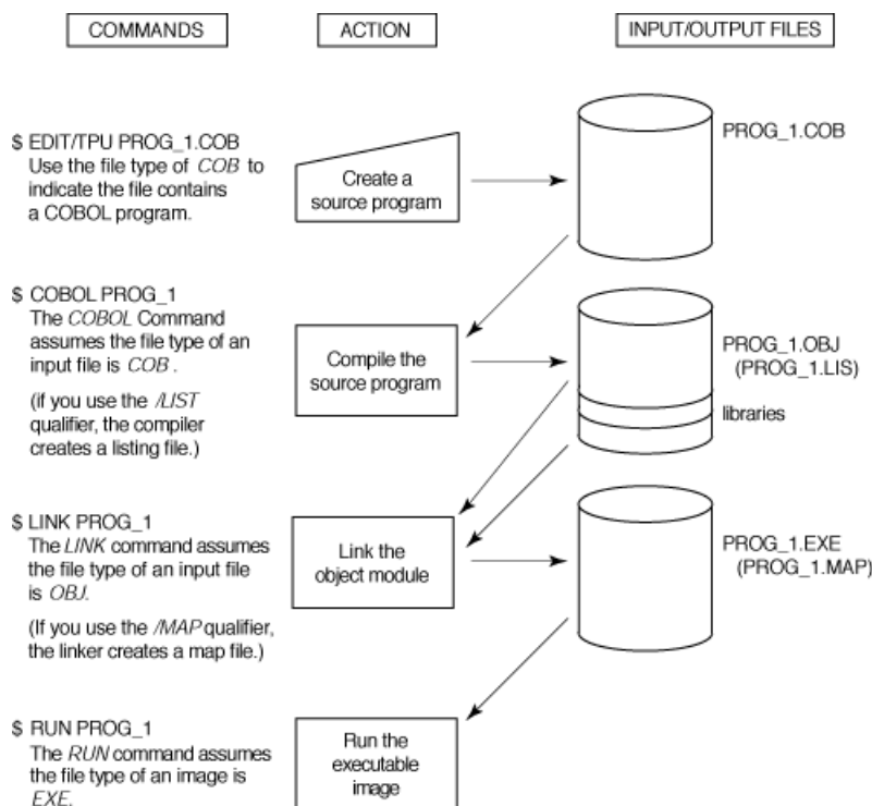
Figure 1.2. DCL Commands for Developing Programs
