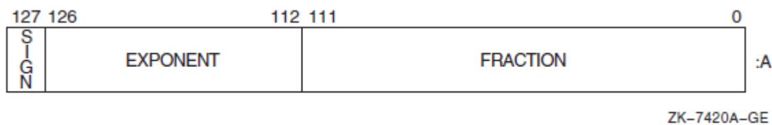
Figure 17.10. XFLOAT Floating-Point Number Format
