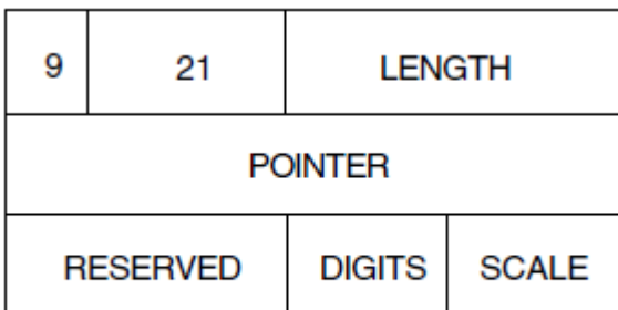
Figure 17.13. Decimal Scalar String Descriptor
