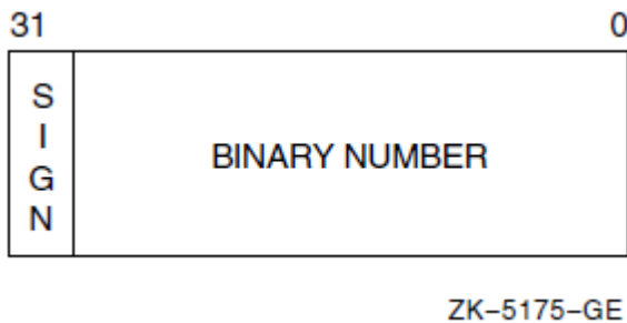
Figure 17.3. Longword Integer Format
