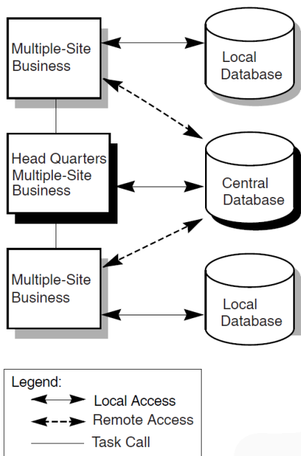
Figure 4.4. A Multiple-Site Business with Multiple-Site Databases
