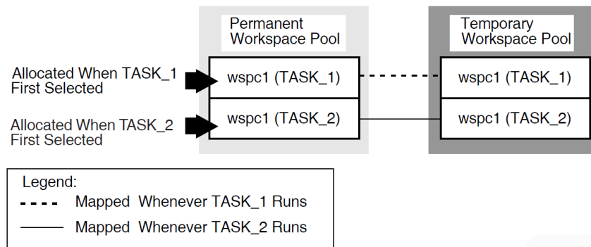
Figure 6.4. Declaring Group Workspaces in the Task Group Definition
