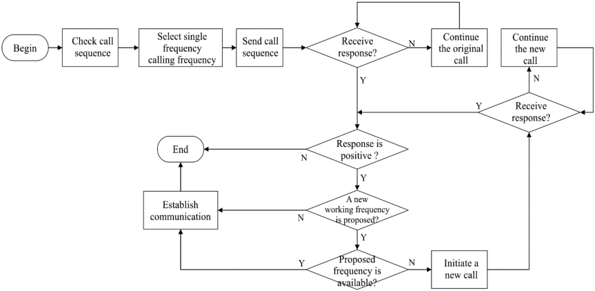
FIGURE A2-3 Procedure for ship station which initiates call to coast station
