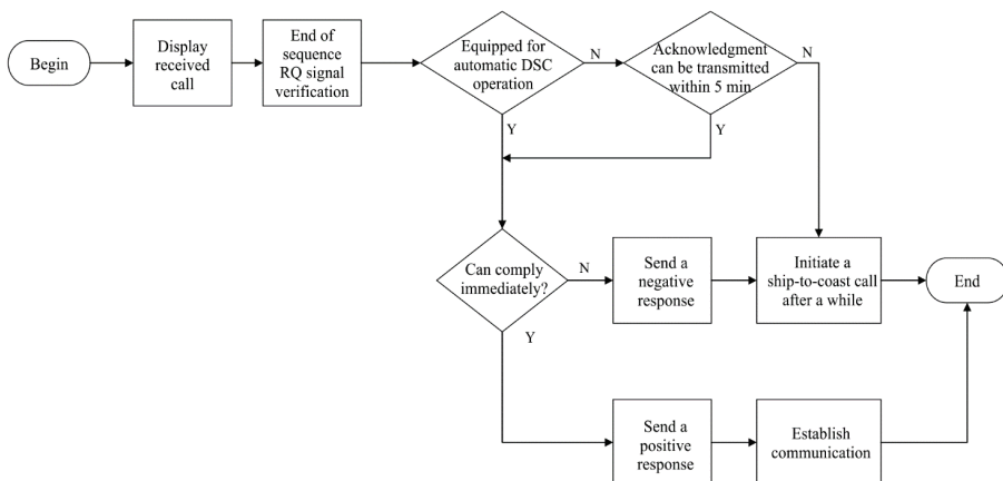
FIGURE A2-2 Procedure for ship station which receives call from coast station
