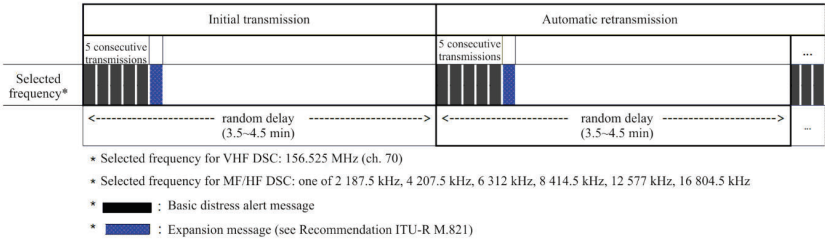
FIGURE A1-1 Single-frequency call attempts
