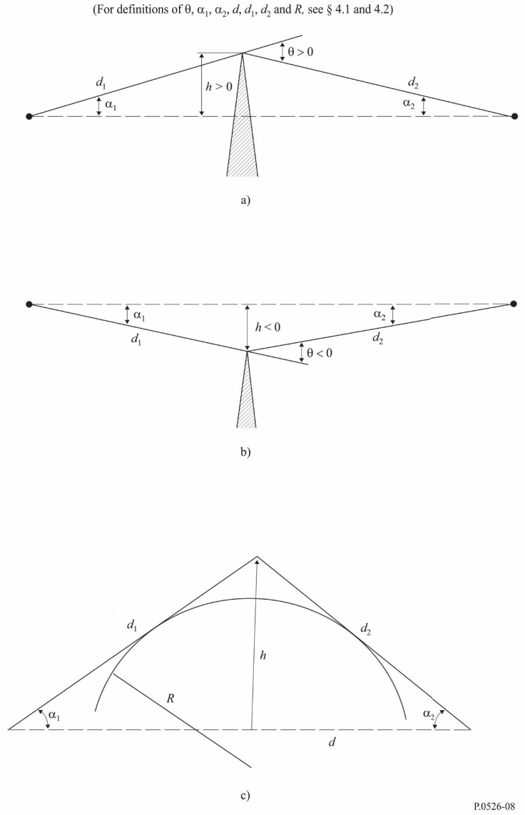
FIGURE 8 Geometrical elements
