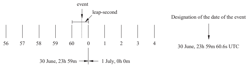
FIGURE 3 Positive leap-second
