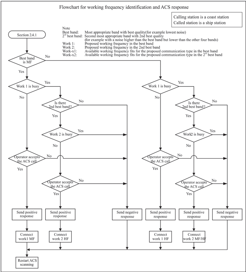
Flowchart for the working frequency identification and following ACS response for the called station when calling station is a coast station and called station is a ship station
