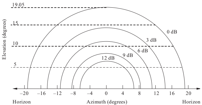
FIGURE 1 The effect of a source of interference at the detrimental level for the RAS, on the horizon at zero azimuth
