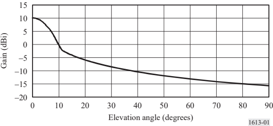
FIGURE 1 Base station antenna pattern
