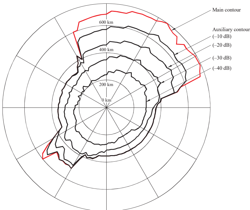
FIGURE 10 (WRC-03) Propagation mode (1) main contour and auxiliary contours
