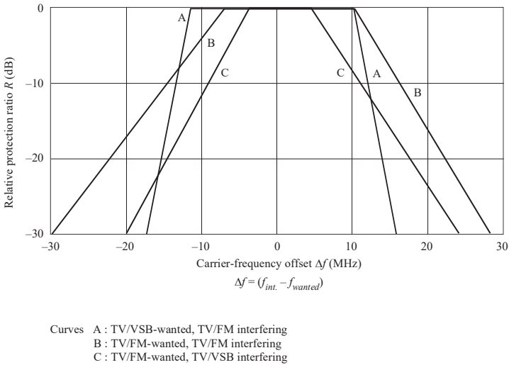
FIGURE 1 Reference case protection ratios relative to co-channel values
