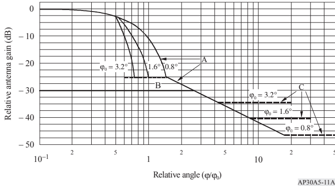
FIGURE 11A Reference patterns for co-polar and cross-polar components for satellite transmitting antennas with roll-off in the main beam for Region 2
