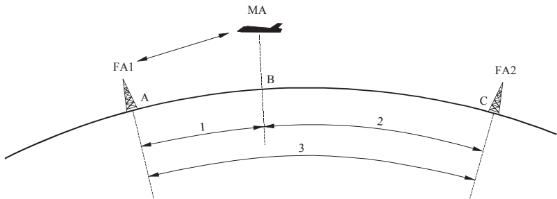
FIGURE 1 Service range, interference range, repetition distance
