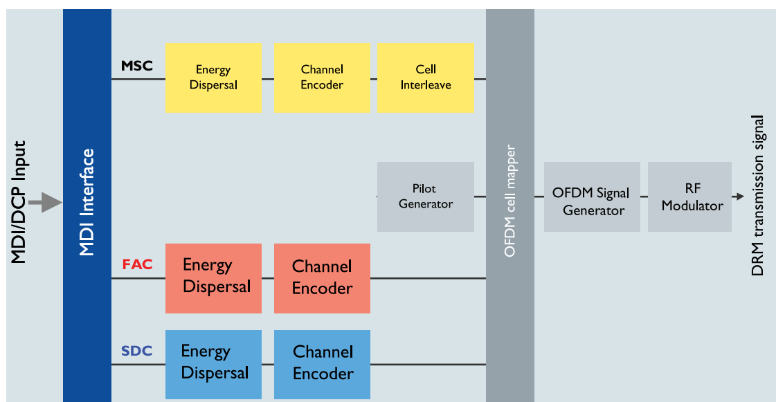
Figure 5.2.3: Conceptual Block diagram of DRM Modulator
