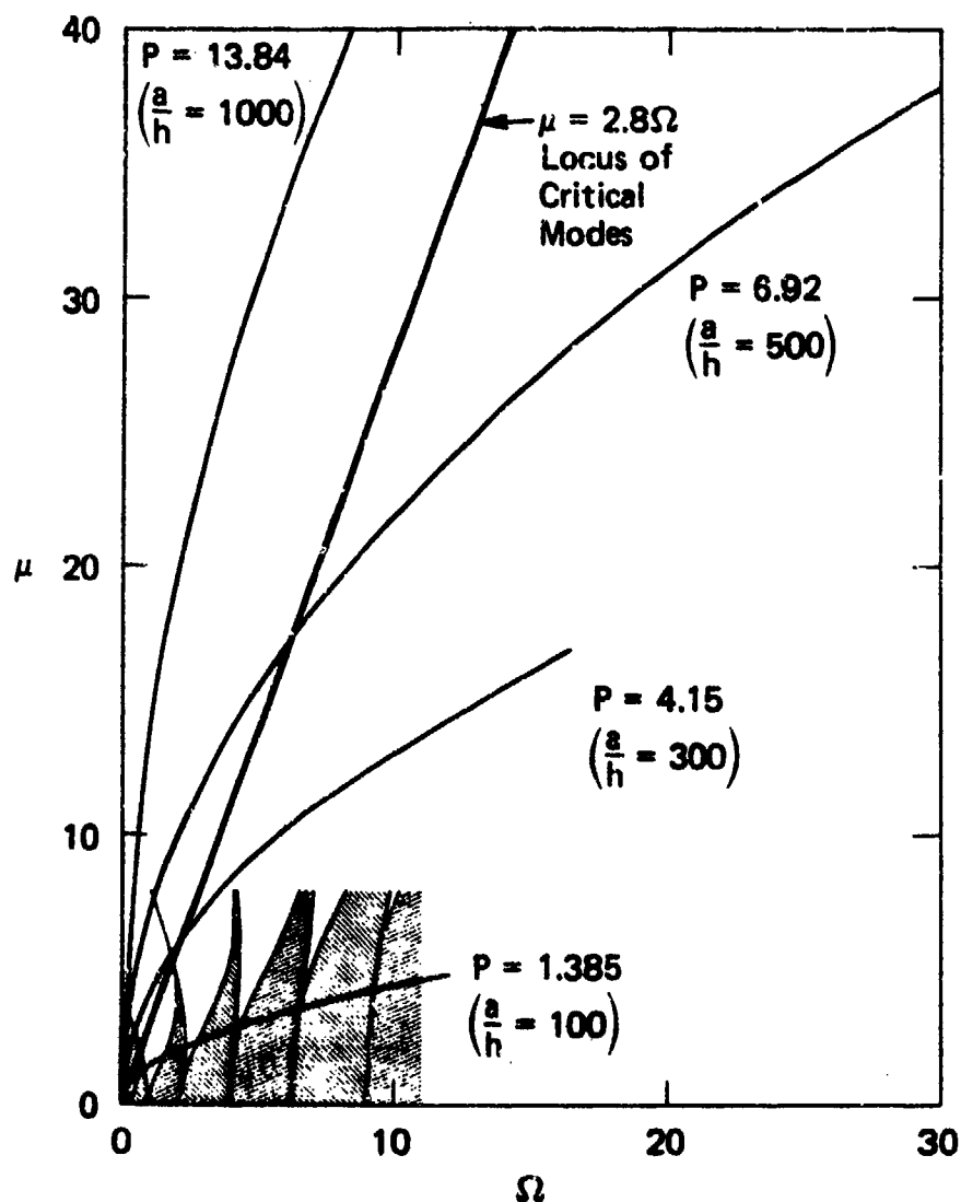
FIGURE 3.26 LOCI OF FLEXURAL MODES ON MATHIEU STABILITY CHART
