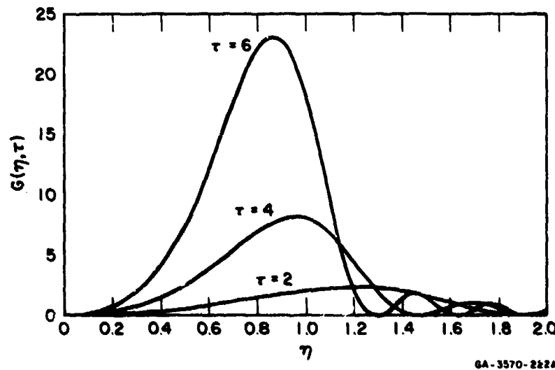
FIGURE 2.3 AMPLIFICATION FUNCTION
