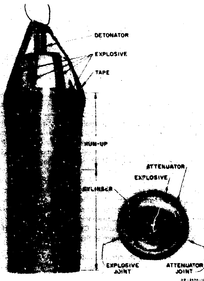
FIGURE 3.12 EXPERIMENTAL ARRANGEMENT
