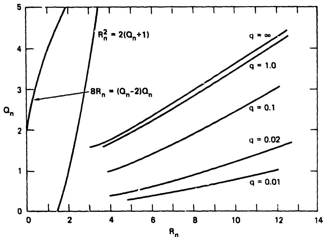
FIGURE 4.8 Q_n vs R_n FOR PREFERRED MODE NUMBER (No Strain Hardening Moment: q = \infty ; No Direction Moment: q = 0 )
