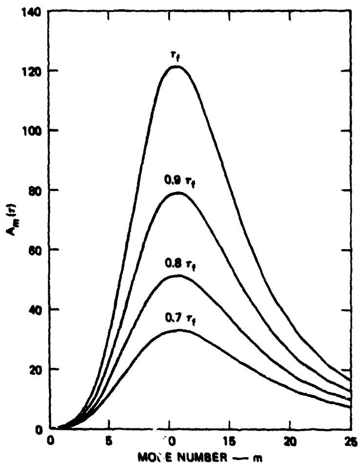
FIGURE 6.2 AMPLIFICATION FUNCTIONS FROM INITIAL DEFLECTIONS
