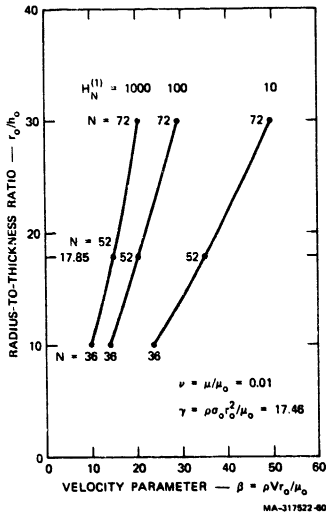
FIGURE 4.35 CRITICAL VELOCITY CURVES ( \nu = 0.01 )
