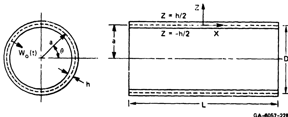
FIGURE 4.1 CYLINDRICAL SHELL — COORDINATES AND DIMENSIONS
