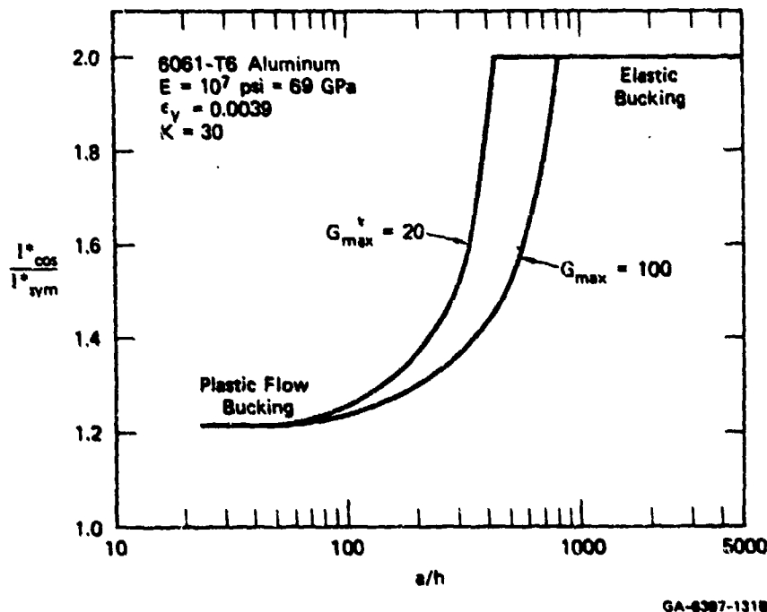
FIGURE 3.34 RATIO OF CRITICAL PEAK COSINE AND SYMMETRIC IMPULSE VERSUS RADIUS-TO-THICKNESS RATIO
