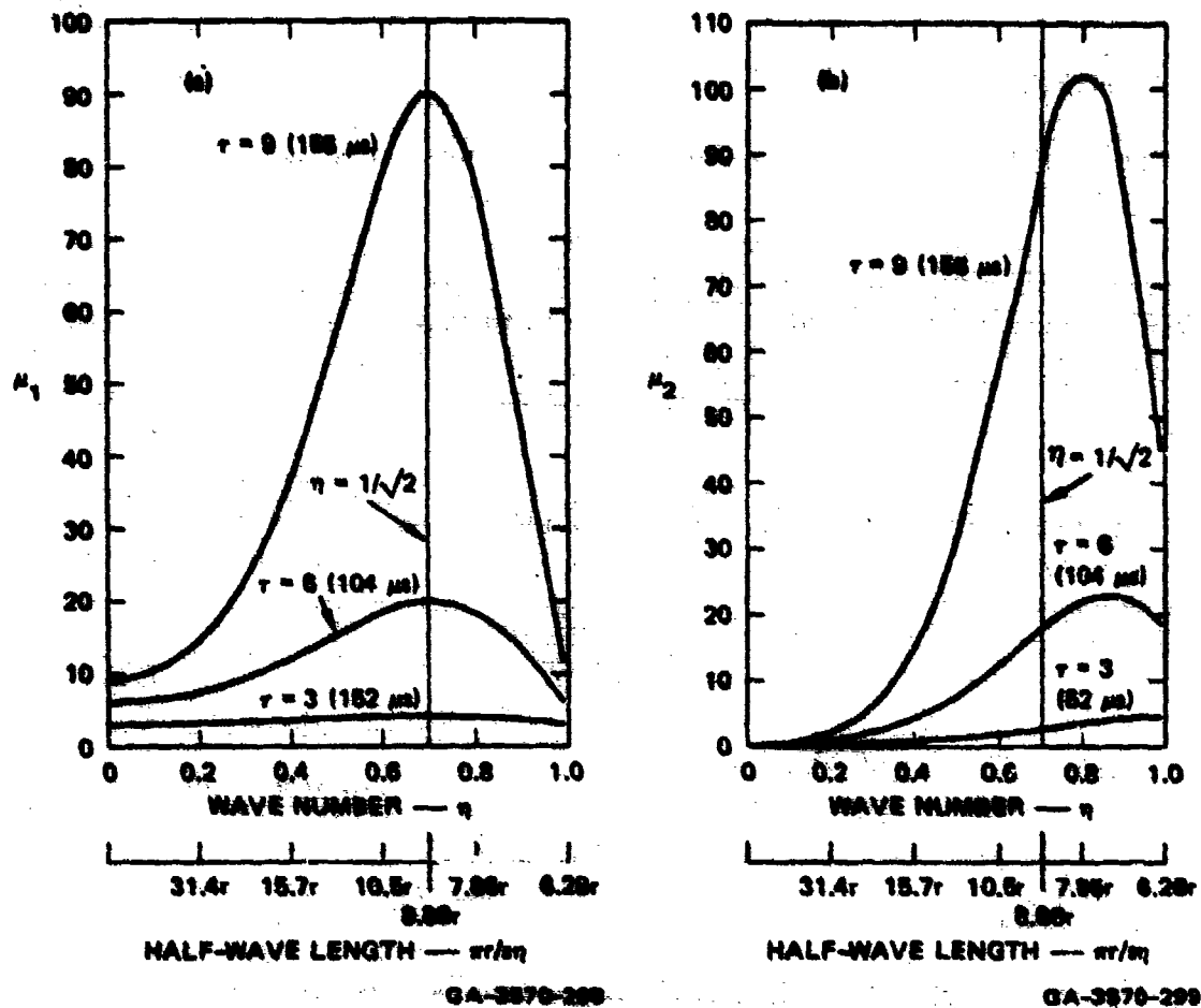
FIGURE 2.28 HYPERBOLIC MAGNIFICATION FACTOR FOR INITIAL VELOCITY [IN (a)] AND DISPLACEMENT [IN (b)] PERTURBATIONS Times are in \mu s for rods in Figure 2.22.
