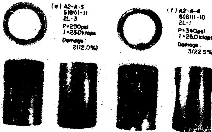
FIGURE 3.56 INCREASING DAMAGE TO SHELLS WITH a/h = 61 , L/a = 2 SUBJECTED TO ASYMMETRIC LOADS. (a-c) QUASI-IMPULSIVE AND (d-f) QUASI-STATIC (psi x 6.9 = kPa, ktaps x 100 = Pa-s)
