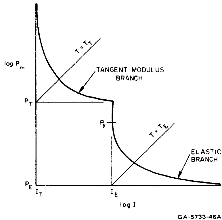
FIGURE 3.51 CHARACTERIZATION OF CRITICAL CURVES FOR BUCKLING
