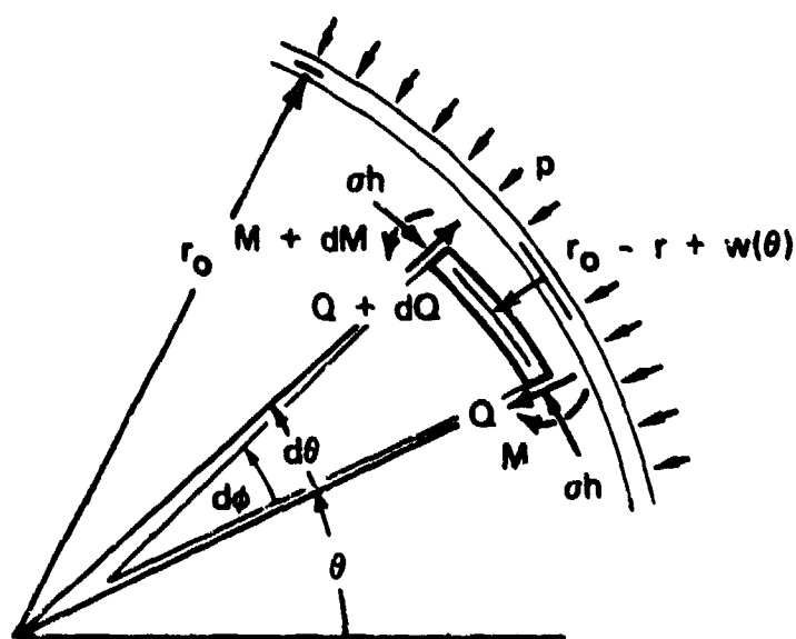
FIGURE 4.26 NOTATION OF RING ELEMENT IN MOTION
