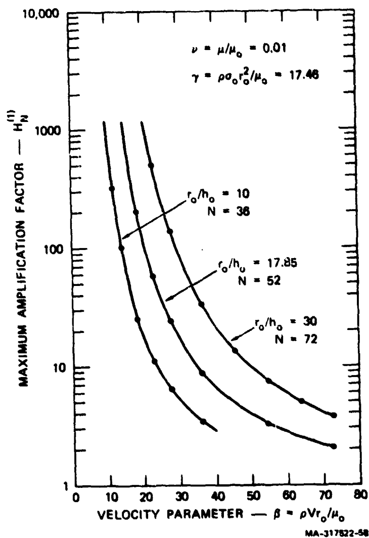
FIGURE 4.33 RELATIONSHIP BETWEEN MAXIMUM AMPLIFICATION FACTOR AND VELOCITY ( \nu = 0.01 )
