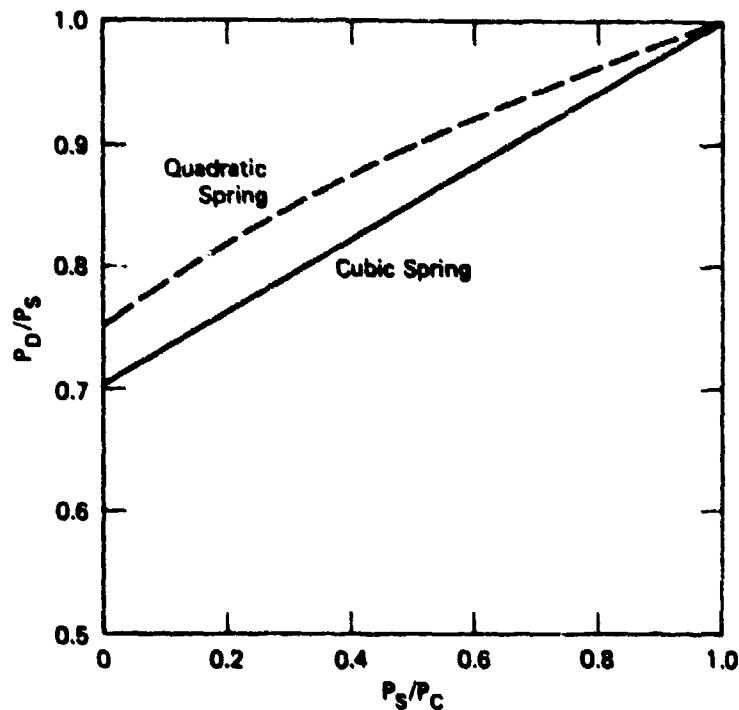
FIGURE 5.11 DYNAMIC BUCKLING LOADS FOR RIGID-ROD COLUMN MODELS
