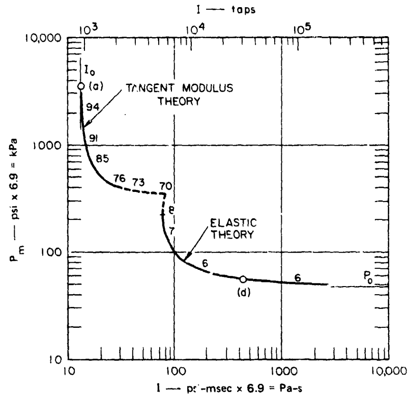
FIGURE 3.45 CRITICAL CURVE FOR BUCKLING OF SHELLS IN FIGURE 3.36 (exponential pulses, 6061-T6 aluminum, a = 3 inches = 76 mm, a/h = 100 , L/a = 2 )
